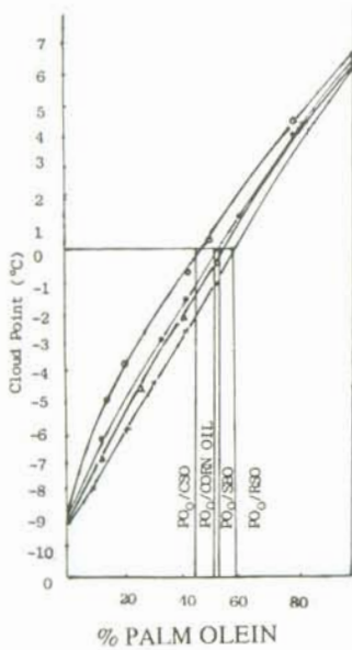
Figure 1. Cloud Points of Blends of Vegetable Oils with Single Fractionated Palm Olein (The cloud point of the unblended palm olein was 7° - 8°C. CSO = cotton seed oil; SBO = soya bean oil; RSO = rape seed oil).
